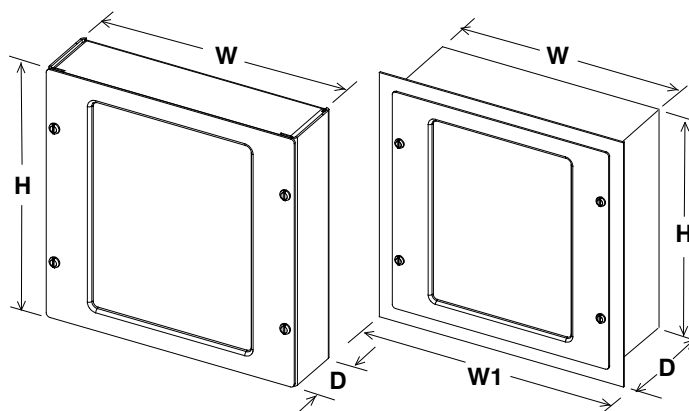
Surface Mounted
